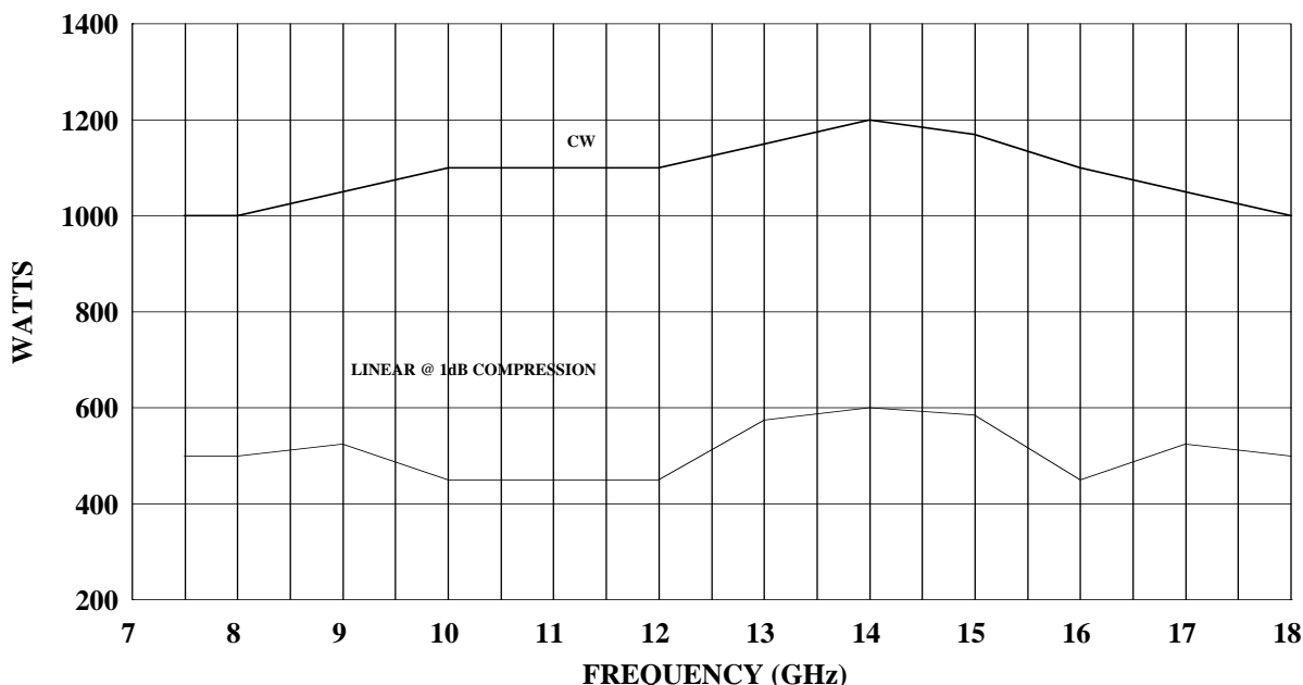
1000T8G18B TYPICAL POWER OUTPUT
